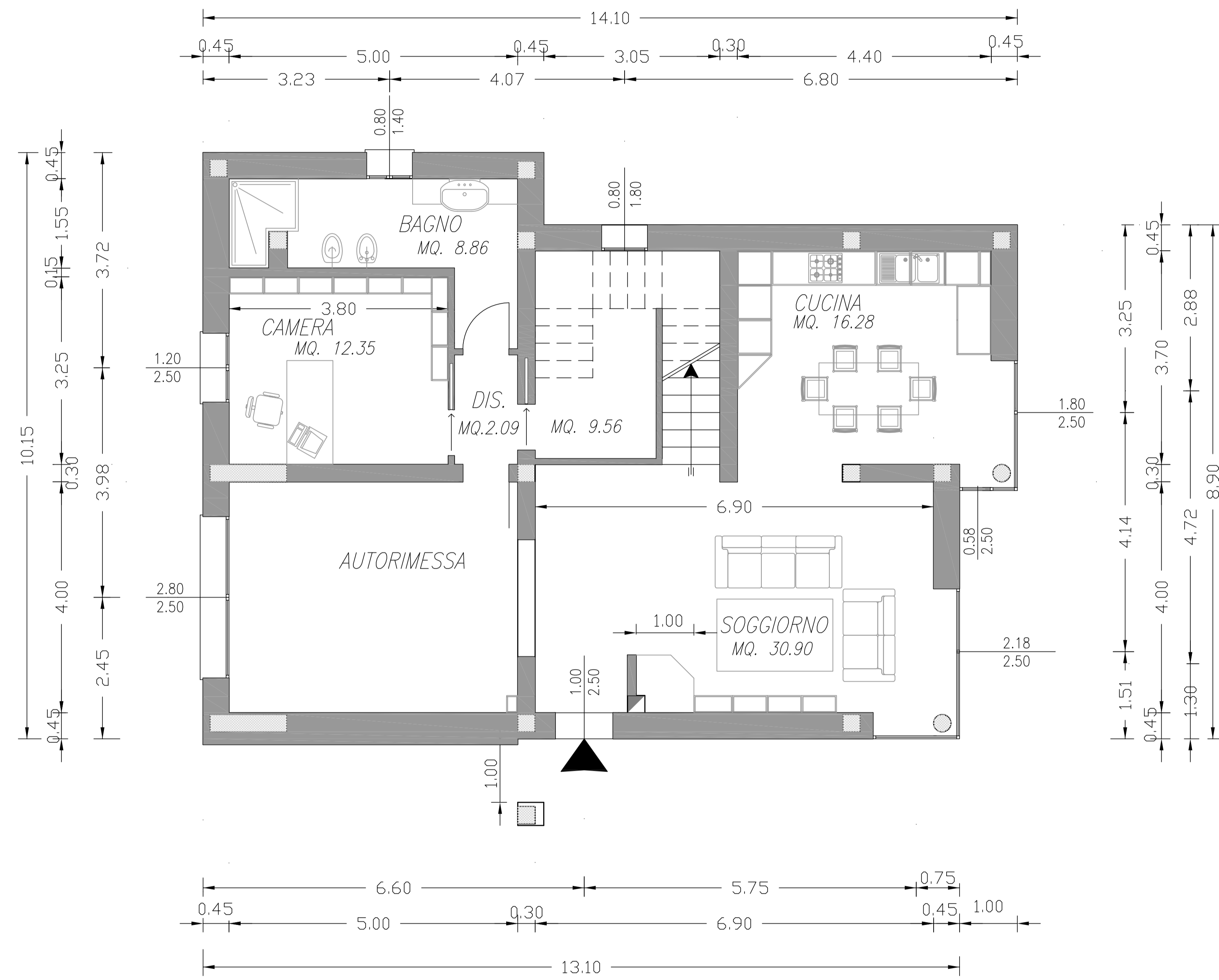
Piano Terra - H=2.80
